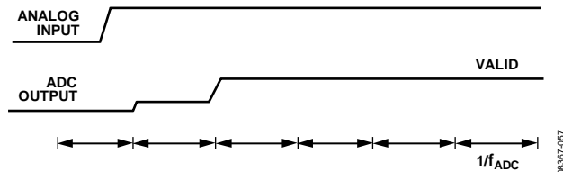
Figure 63. Step Change on Analog Input, Sinc 3 Filter
