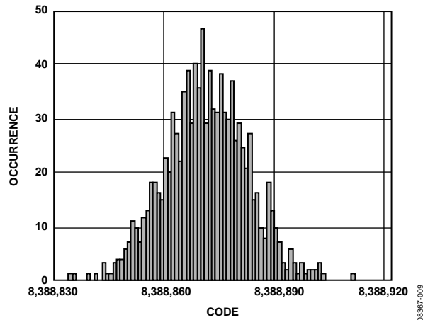
Figure 10. Noise Distribution Histogram ( V_{REF} = AV_{DD} = 5\text{ V} , Output Data Rate = 2400 Hz, Gain = 1, Chop Disabled, \text{Sinc}^4 Filter)
