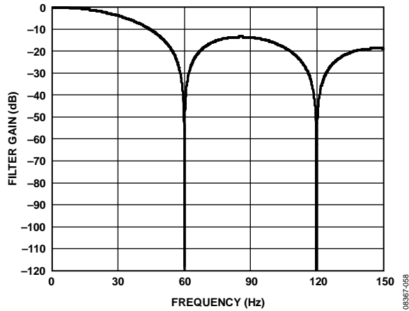
Figure 65. Filter Response for Average + Decimate Filter (Sinc 2 Filter, FS[9:0] = 5, Average by 16)
