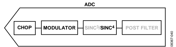
Figure 44. Chop Enabled
