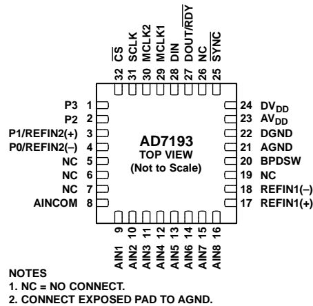
Figure 6. 32-Lead LFCSP Pin Configuration
